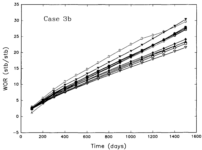
Figure 14: Water-oil ratio for Case 3b
