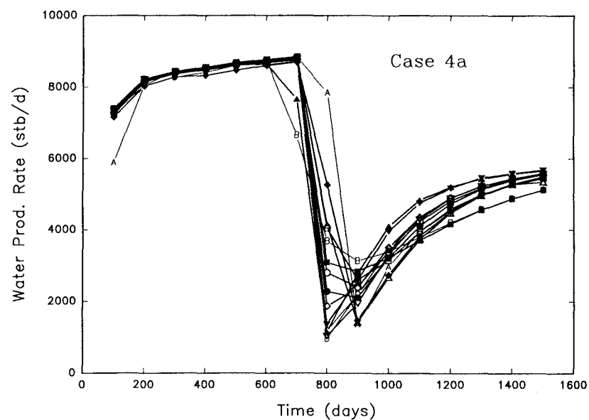
Figure 20: Water production rate for Case 4a
