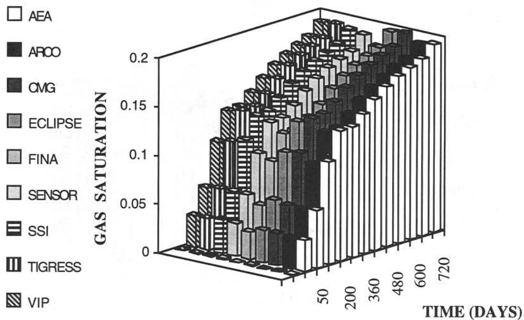
FIGURE 12: COMPARISON OF GAS SATURATIONS AT 1,13,1
