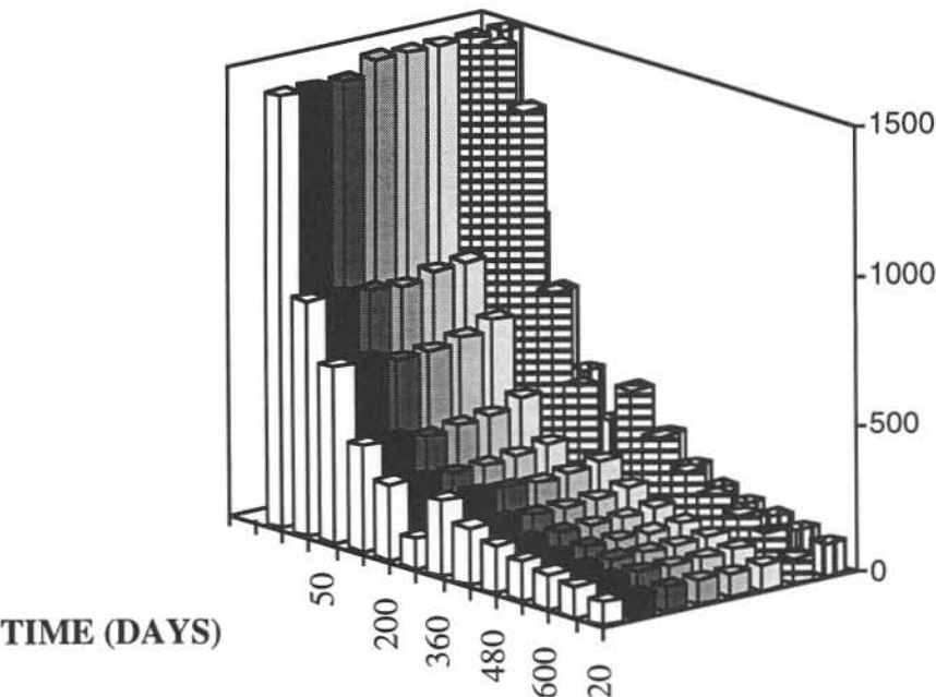
FIGURE 15: COMPARISON OF OIL RATES FOR WELL 21
