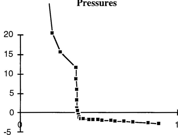
Figure 1: Water-Oil Capillary Pressures
