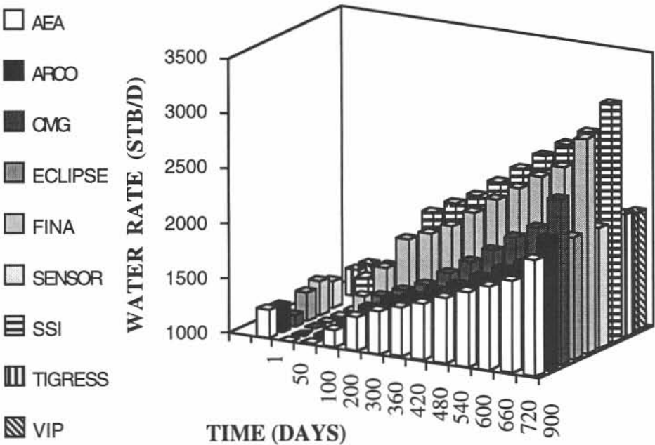
FIGURE 14: COMPARISON OF WATER INJECTION RATES
