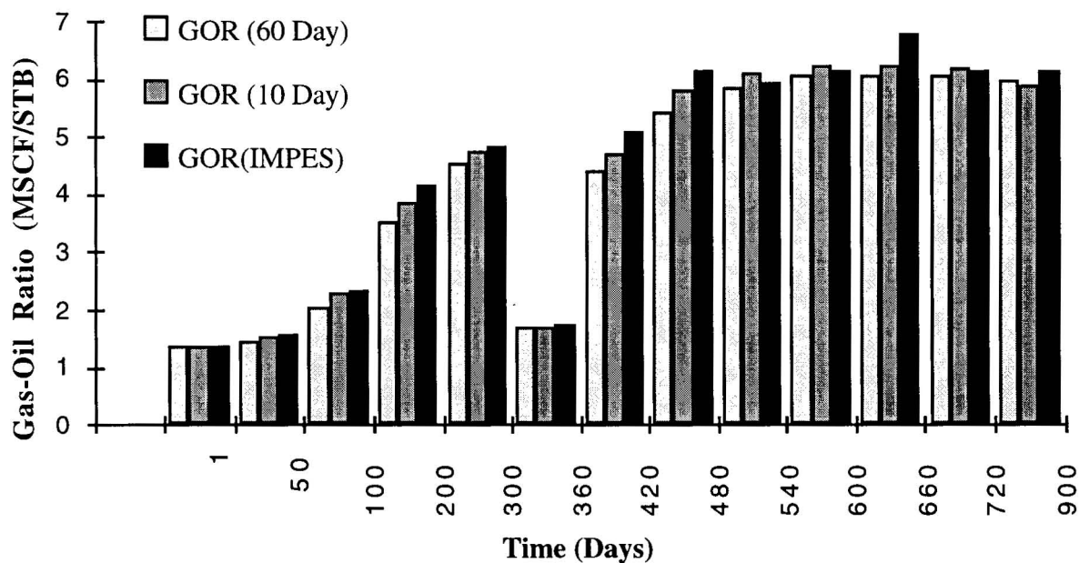
Figure 7: Variation of GOR With Time Step
