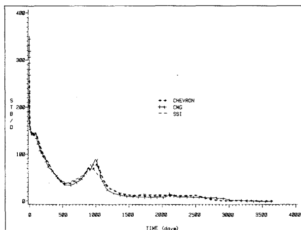
Fig. 15—Problem 3: oil rate for far producer (full-well basis).
