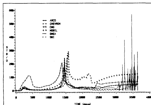
Fig. 9—Problem 2: water rate for far producer (full-well basis).
