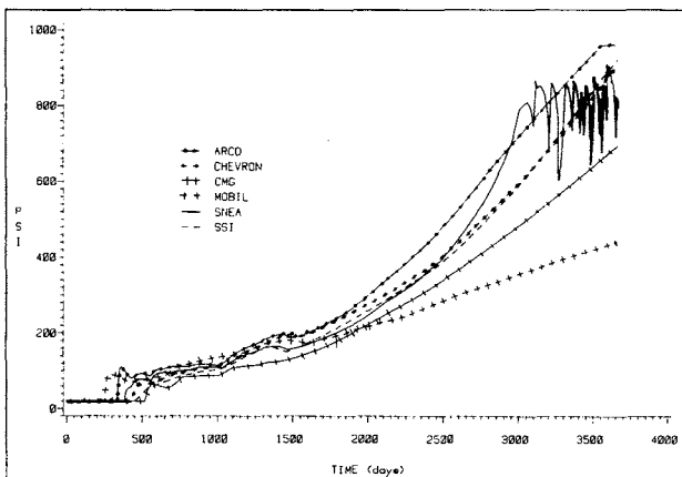
Fig. 10—Problem 2: BHP for near producer.
