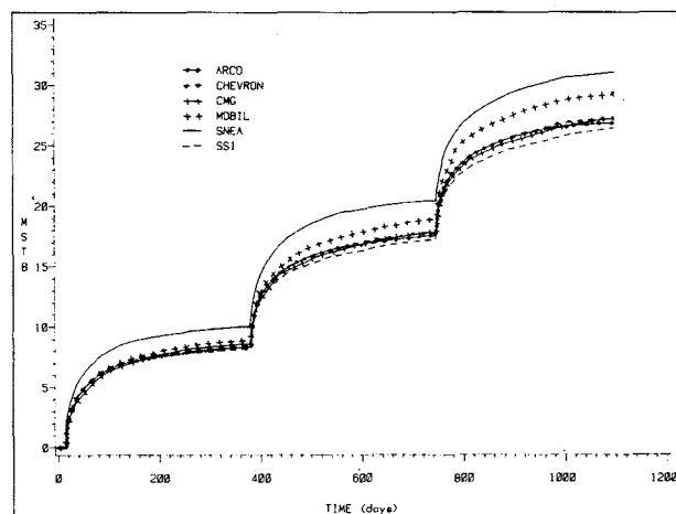
Fig. 3—Problem 1: cumulative water production.
