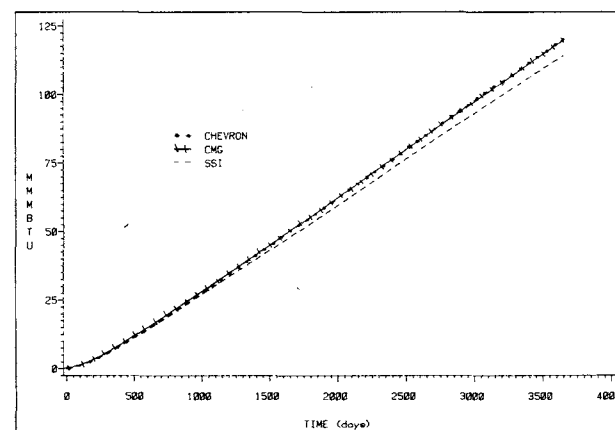
Fig. 21—Problem 3: cumulative heat loss for full pattern.
