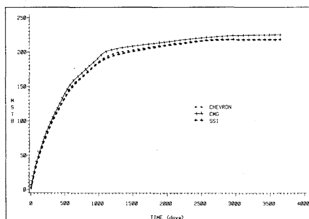
Fig. 19—Problem 3: cumulative oil production for full pattern.
