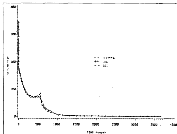
Fig. 14—Problem 3: oil rate for near producer (full-well basis).
