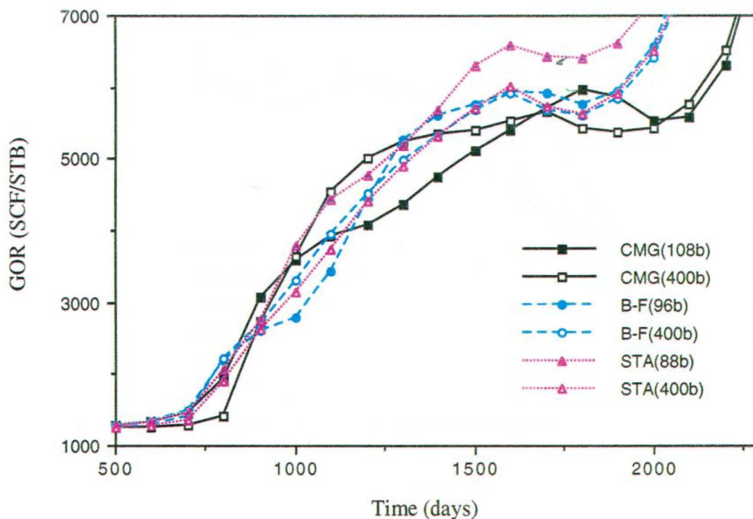
Fig.12 - Producer 1 Gas/Oil Ratio
