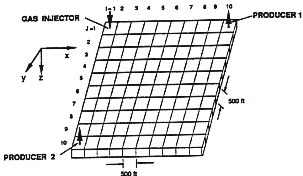
Fig. 1 - Reservoir and grid system
